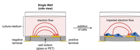
Figure 8: Schematic cross-sectional view of wells in the E-plates used in the real-time cell analysis system, cell presence changes the impedance between the electrodes.
