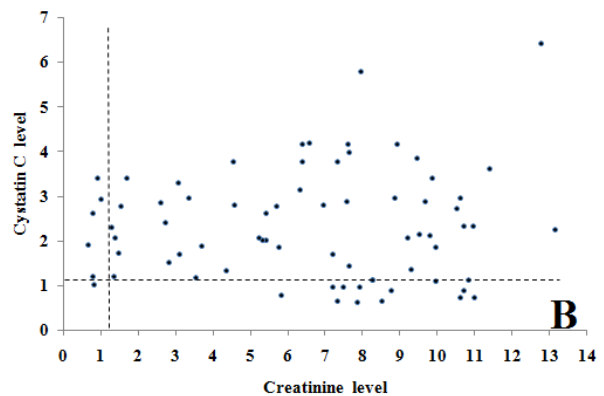
Figure 4: Scatter diagram showing the correlation between creatinine and cystatin C in the male patient group (A) and in the females (B). The dotted lines represent the optimal cut off values of creatinine and cystatin C.
