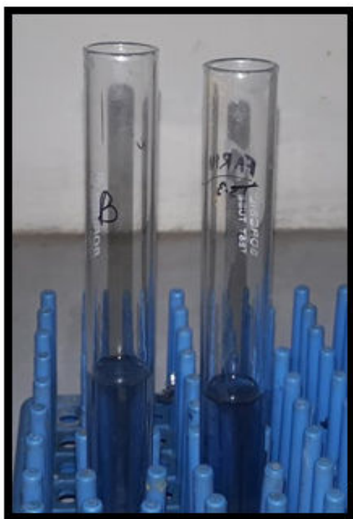
Figure 8: Lowry's assay.
