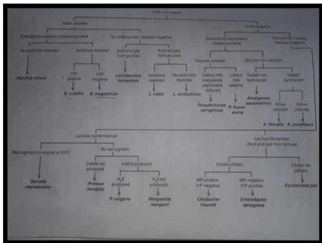
Figure 2: Bergey’s manual.
